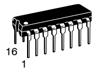
PDIP-16 CASE 648-08
